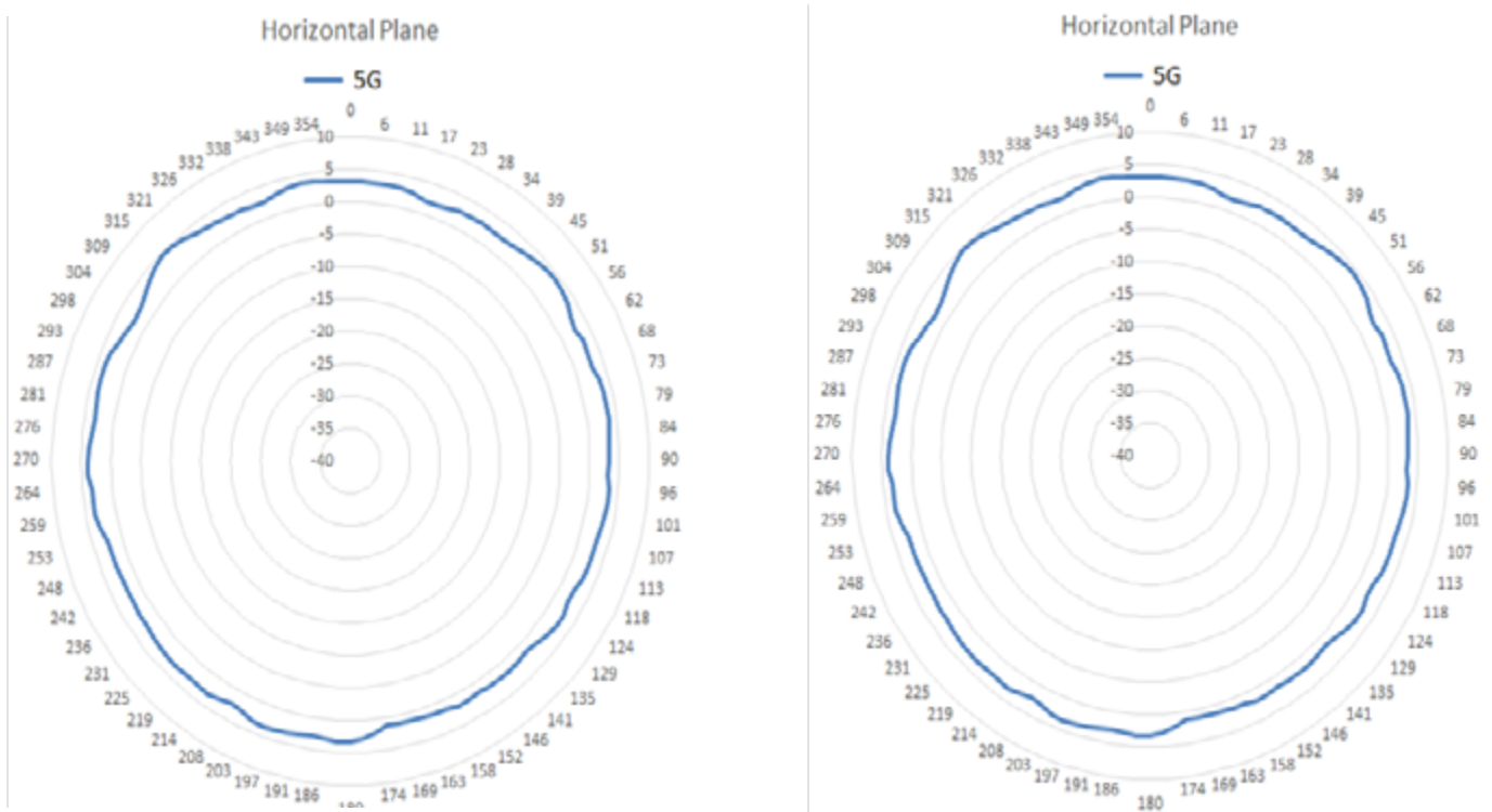
AP505i Antenna Radiation Patterns - 5.0GHz
